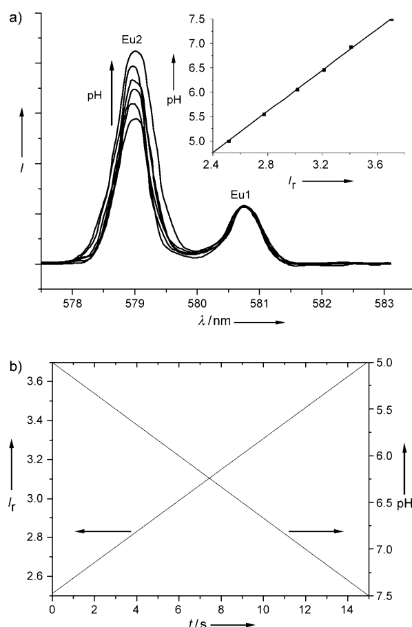
Figure 4. a) Intensity variation of the Eu2 ^5\text{D}_0 \rightarrow ^7\text{F}_0 transition from high (pH 7.5) to low (pH 5) pH values; the inset shows the linear variation of I_r with the pH value. b) Time variation of I_r with the pH change from 5 to 7.5 in ramping mode (measured with a glass electrode).
